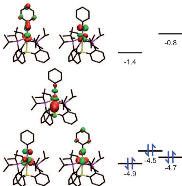
Figure 2. Frontier Kohn–Sham orbitals of [(TPB)Fe≡NPh] calculated at the B3LYP/6-31G(d) level. Energies in electron volts.
